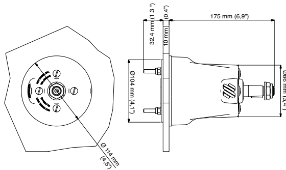
UH32-F and UH40-F dimensions
