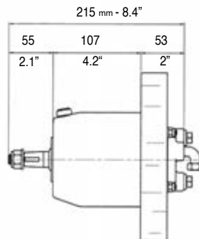
UP25F, UP28F, UP33F, UP39F, UP45F DIMENSIONS
