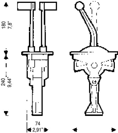
Straight levers B50 B59 with interlock
