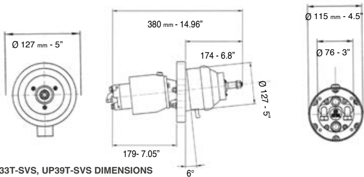
UP28T-SVS, UP33T-SVS, UP39T-SVS DIMENSIONS
