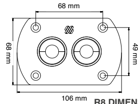
R8 DIMENSIONS
