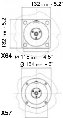
UP25F, UP28F, UP33F, UP39F, UP45F DIMENSIONS
