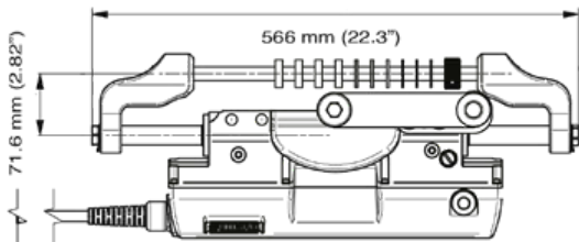
UPA123 - DIMENSIONS
