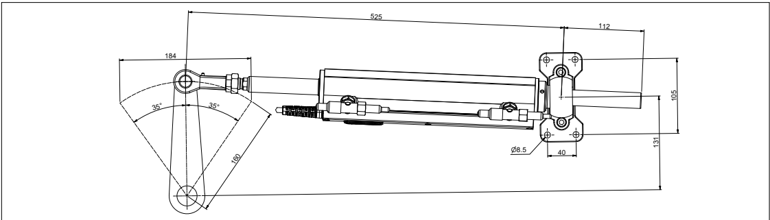
UC120E-I DIMENSIONS
