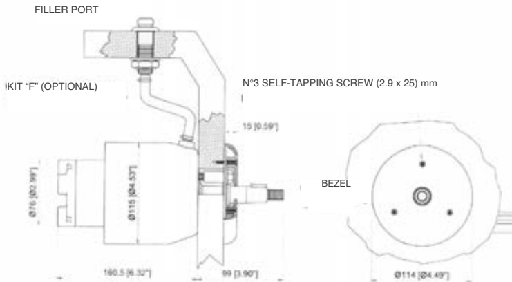
UP28R, UP33R, UP39R, UP45R DIMENSIONS
