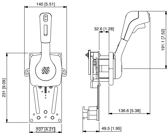
B310CH - B310BR - B310B - B310B-ETC
