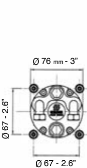
UP25F, UP28F, UP33F, UP39F, UP45F DIMENSIONS
