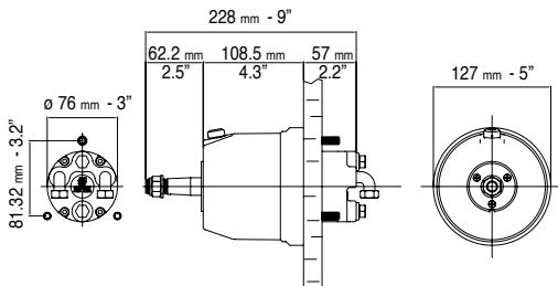
UP25F, UP28F, UP33F, UP39F, UP45F DIMENSIONS
