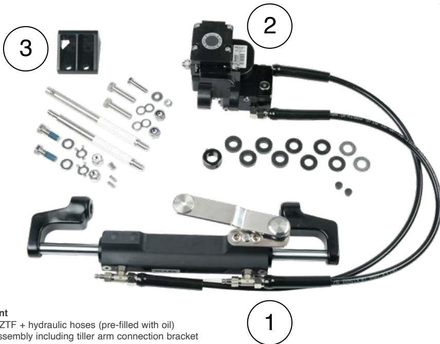
ZTF - Zero torque feedback tiller steering systems
