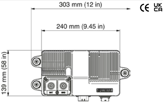
DCDC converter dimensions
