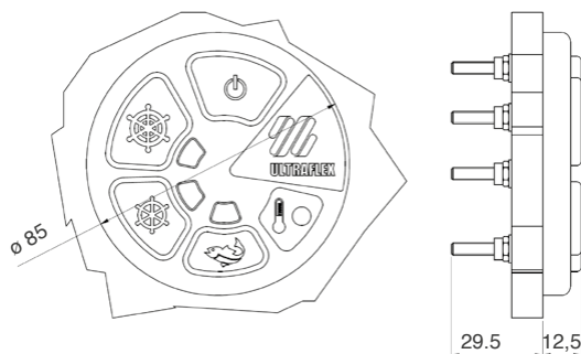
UCMD DIMENSIONS
