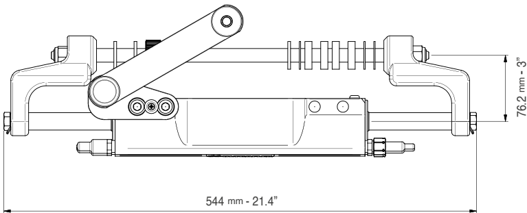
UC130-SVS, UC130P-SVS DIMENSIONS
