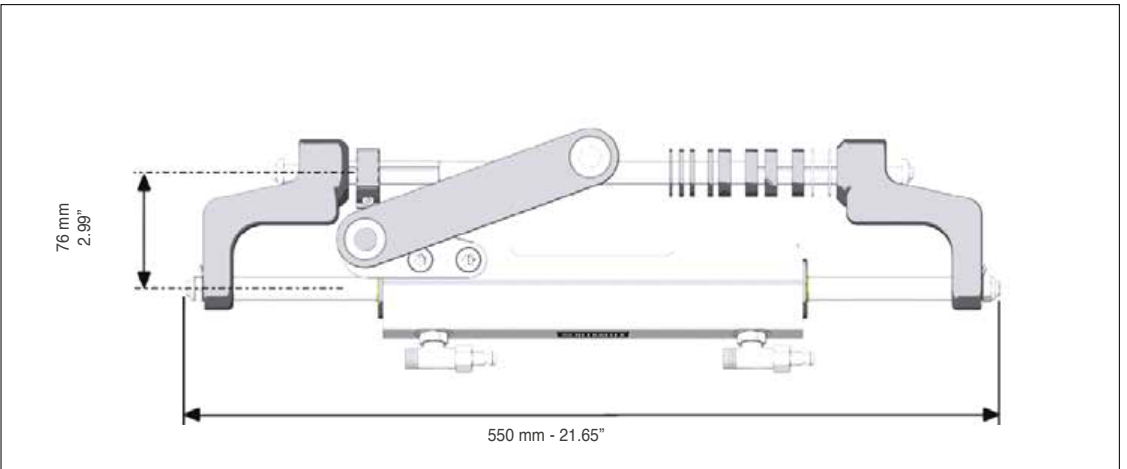
UC95-OBF DIMENSIONS
