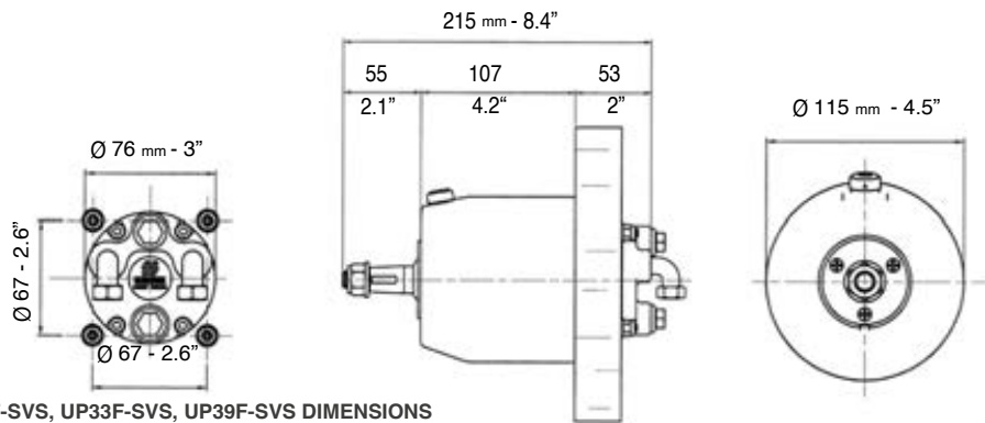
UP28F-SVS, UP33F-SVS, UP39F-SVS DIMENSIONS
