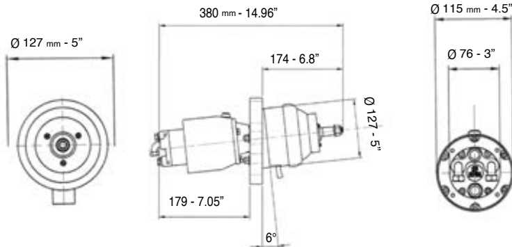
UP25T, UP28T, UP33T, UP39T, UP45T DIMENSIONS
