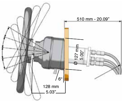
UH32-T and UH40-T dimensions
