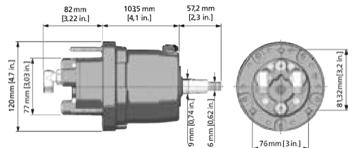
UP20F DIMENSIONS
