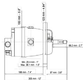
UP56, UP68 REAR MOUNT
