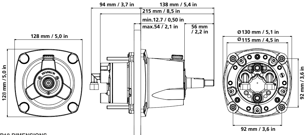
UP18 DIMENSIONS
