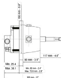
UP56, UP68 INTERMEDIATE MOUNT
